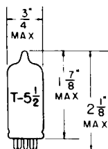
GLASS BULB SMALL BUTTON MINIATURE 7 PIN BASE E7-1 OUTLINE DRAWING JEDEC 4-2
