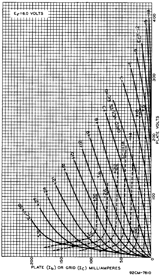
Fig. 2 - Average Plate Characteristics of Type 5893.
