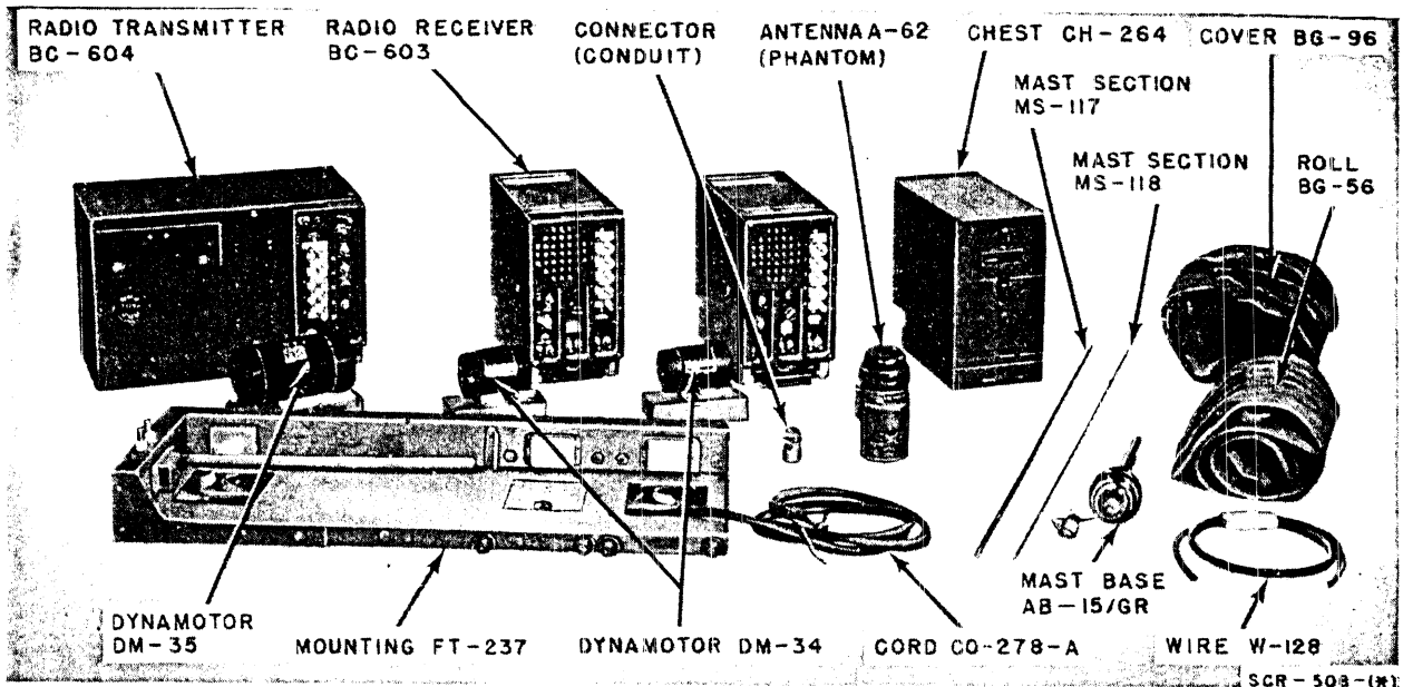
Figure 95. Radio Set SCR-508-(*).
