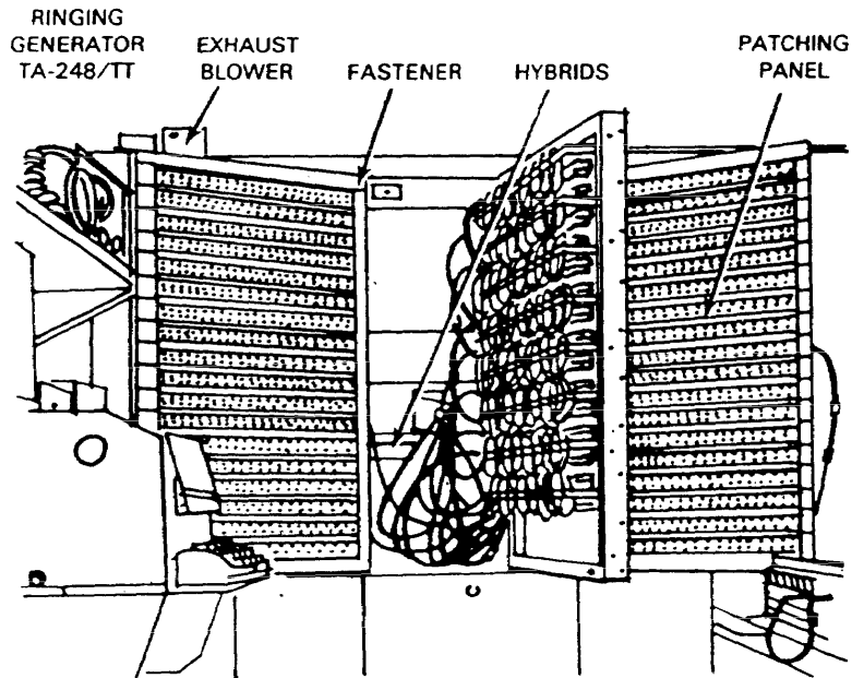
PATCHING PANEL CENTER BAY OPEN FOR MAINTENANCE
