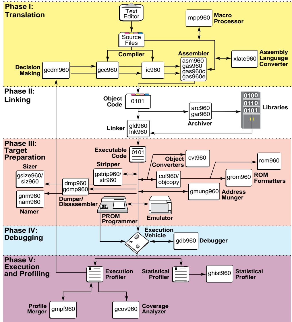
Figure 1-1 CTOOLS Overview
