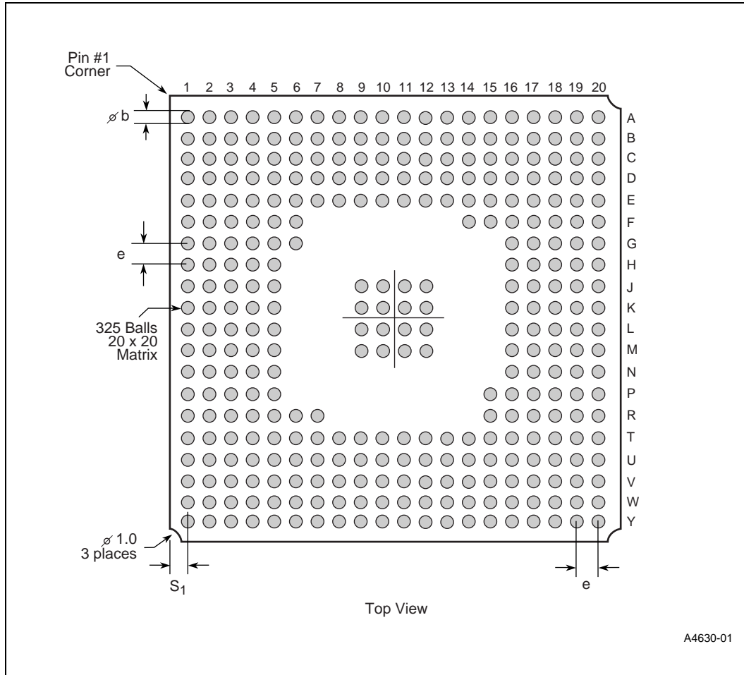
Figure 4. 324-Plastic Ball Grid Array (Top View)
